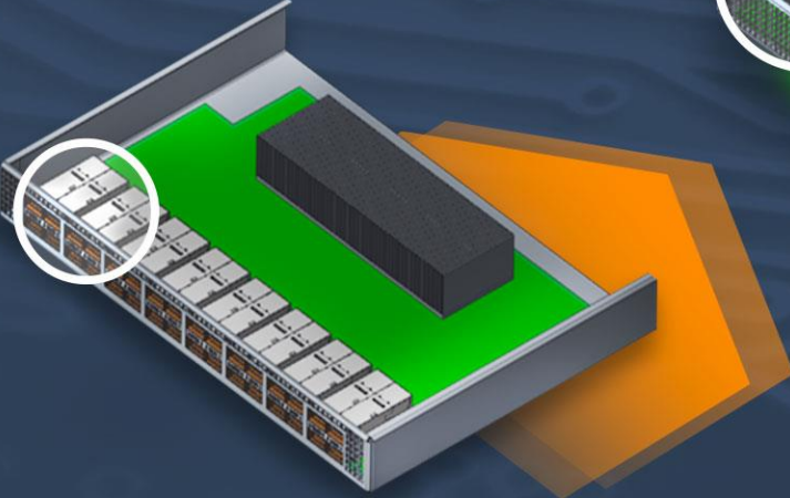
Faceplate Pluggable Optics (OSFP/QSFP-DD)
